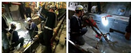
潛盾道版止漏
